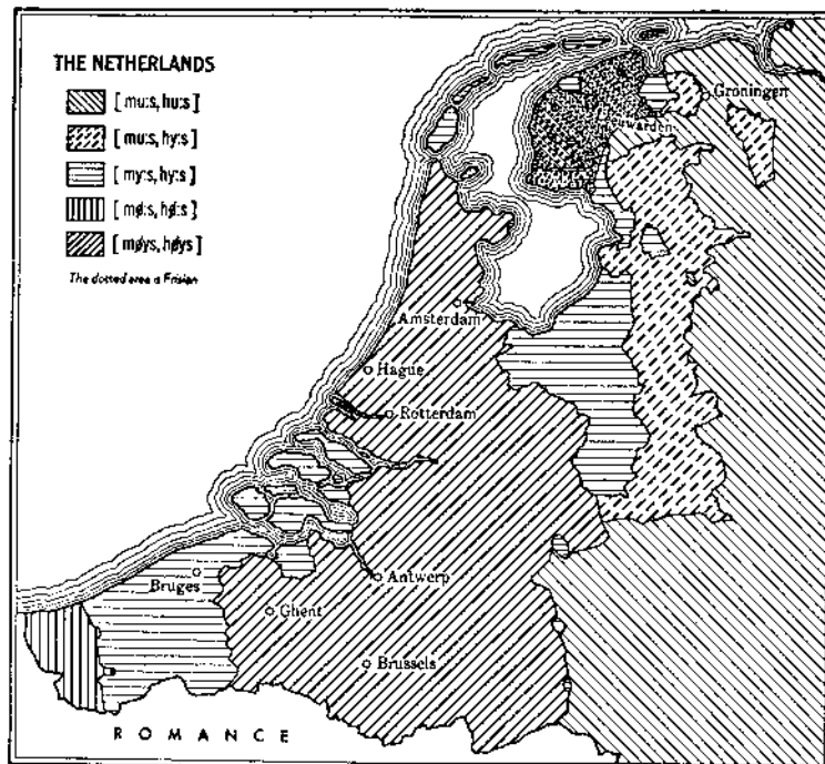
FIGURE 6. Distribution of syllabic sounds in the words mouse and house in the Netherlands. — After Kloetze.
